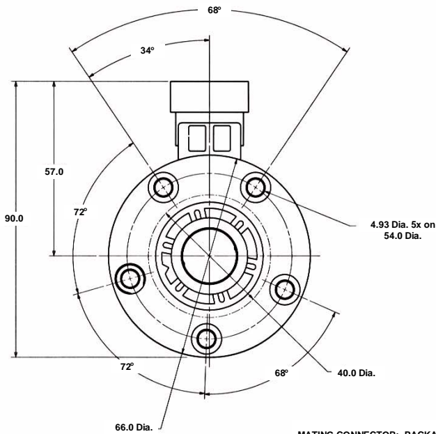
Figure 2 Mounting
